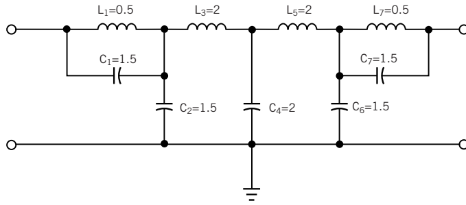
A composite lowpass filter uses four component values.
