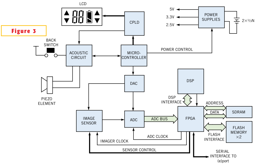
Careful hardware and software partitioning, including reliance on the PC for most of the image processing, optimizes (e)film cost, battery life, and picture quality (courtesy Silicon Film Technologies).
