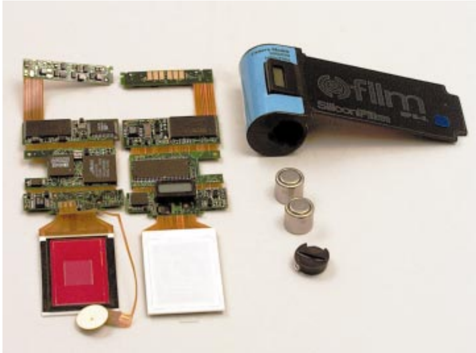
Squeezing two batteries and most of the (e)film's electronics (left) into a film-cartridge-sized form factor requires a mechanical-engineering magic act and manual dexterity (right). The left photo shows views of the pc-board top and bottom; each system requires only one circuit board (courtesy Silicon Film Technologies).
