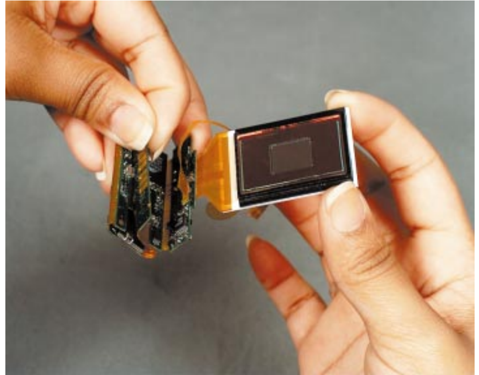
Squeezing two batteries and most of the (e)film's electronics (left) into a film-cartridge-sized form factor requires a mechanical-engineering magic act and manual dexterity (right). The left photo shows views of the pc-board top and bottom; each system requires only one circuit board (courtesy Silicon Film Technologies).
