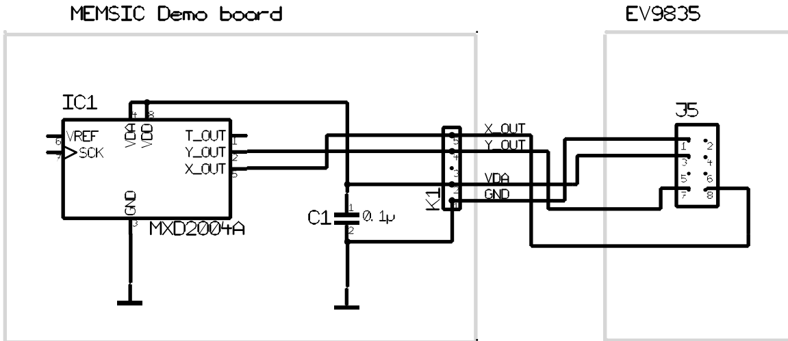
Figure 3 - Schematic Diagram
